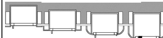
3/8" Flat Trim 1-1/2" Square Trim 2-1/2", 3" Rolled Edge 4" Rolled with Flush Pull or 4-1/2" w/Std Pull
