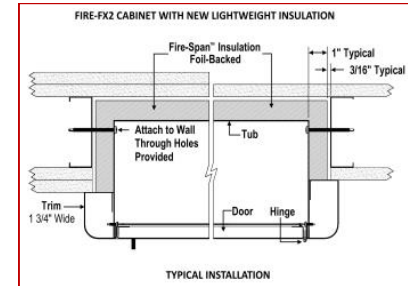
FIRE-FX2 CABINET WITH NEW LIGHTWEIGHT INSULATION Attach to Wall Through Holes Provided Trim 1 3/4" Wide 1" Typical 3/16" Typical TYPICAL INSTALLATION Black Vertical FE Letters LDCVBF E Red Vertical FE Letters LDCVRF E White Vertical FE Letters LDCVWF E Black Horizontal FE Letters LDCHBF E Red Horizontal FE Letters LDCHRF E White Horizontal FE Letters LDCHWF E Lettering: Etched on Glass, Engraving on Metal, Silkscreen; Not Available for #7 or #8 Finish on Doors. Check Box and Attach Separate Submittal to Order.
