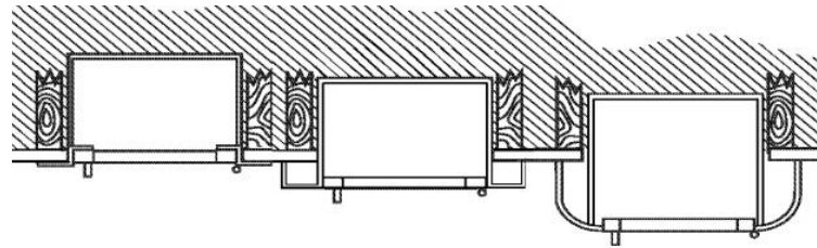
3/8" (.9cm) FLAT TRIM
