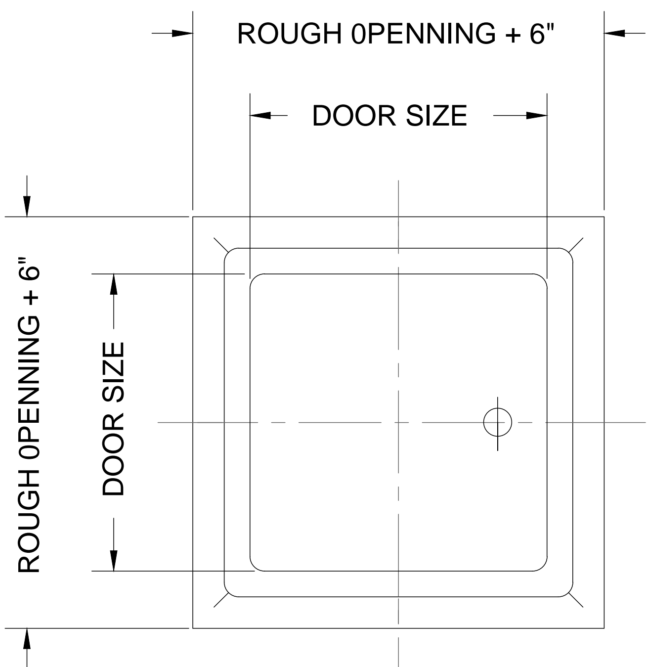
Access Panel -Type Panel Elevations
