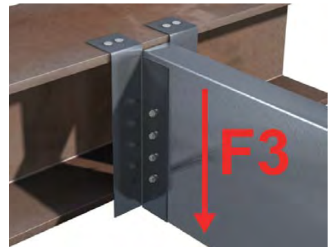
Load Direction
