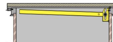
Stowed Position
