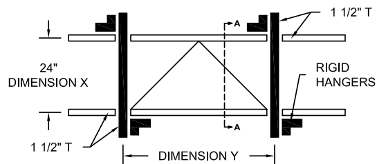
PANEL SUPPORT ILLUSTRATION
