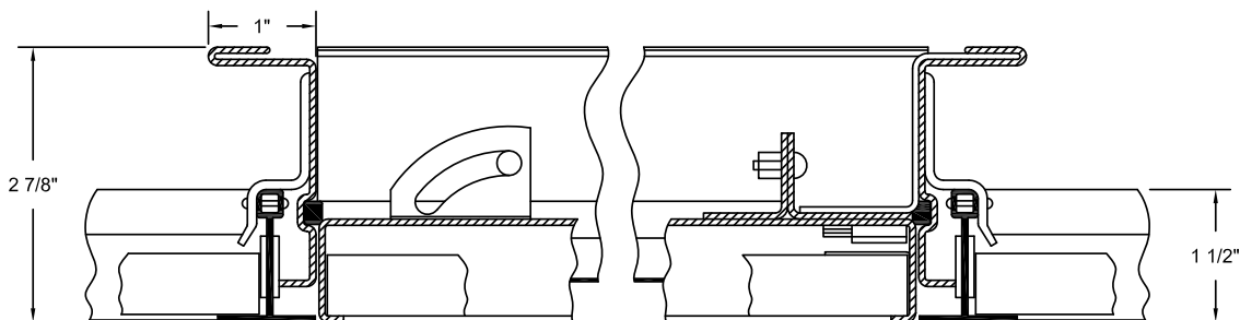
PANEL SUPPORT ILLUSTRATION
