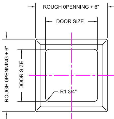
Drop-in Access Panel -Type Panel Elevations
