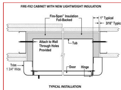
TYPICAL INSTALLATION
