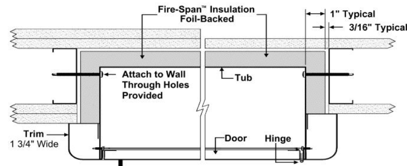
TYPICAL INSTALLATION
