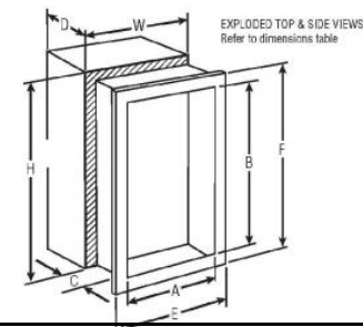
1483F12SI in Silver Finish
