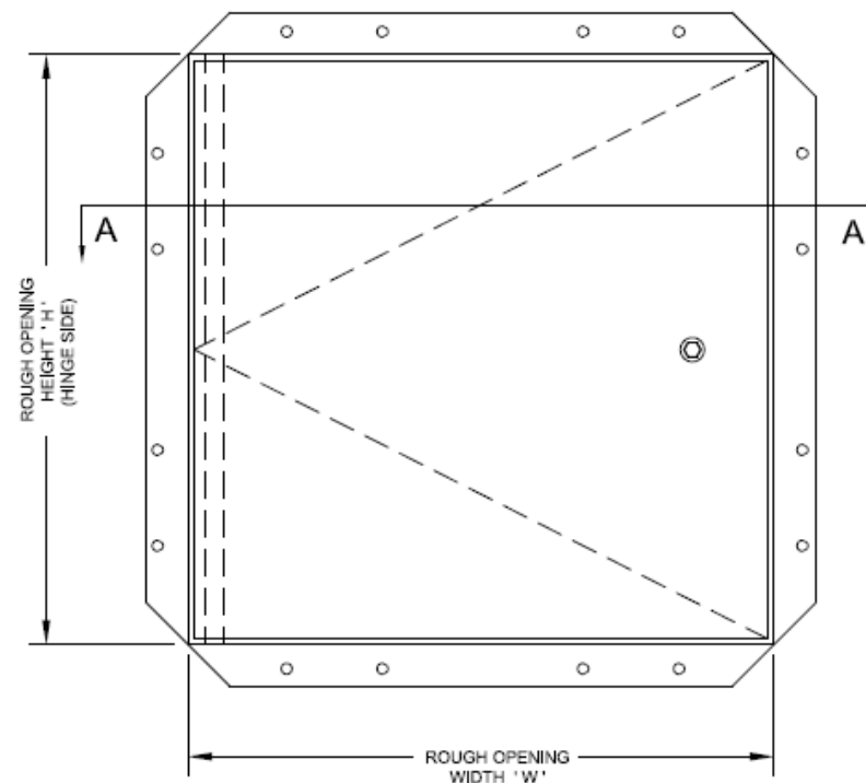
FRONT ELEVATION
